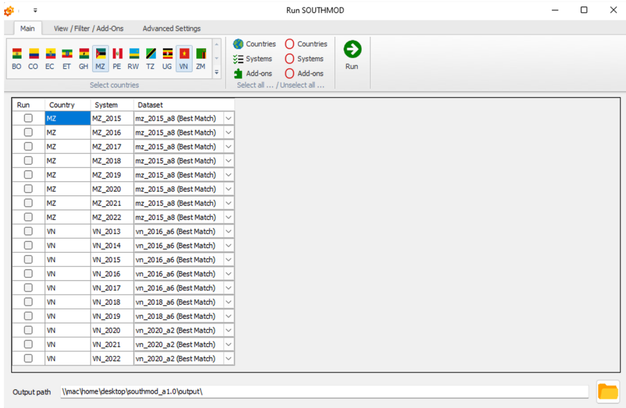
Figure 8.2: The 'Run SOUTHMOD' dialog: Example from VNMOD and MOZMOD
