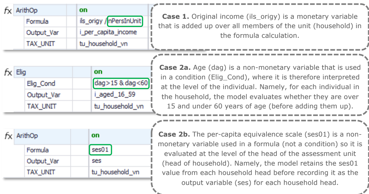
Figure 5.4: Interpreting conditions with respect to assessment units: Examples from VNM0D
