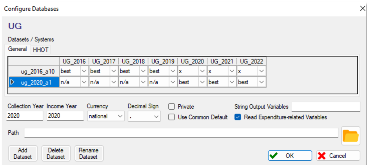
Figure 4.7: The 'Configure Databases' dialog: Example from UGAMOD
